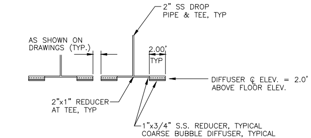
1 COARSE BUBBLE MIXER DETAIL (TYP) NOT TO SCALE
