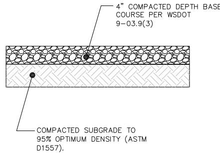
5 GRAVEL SURFACING SECTION NOT TO SCALE
