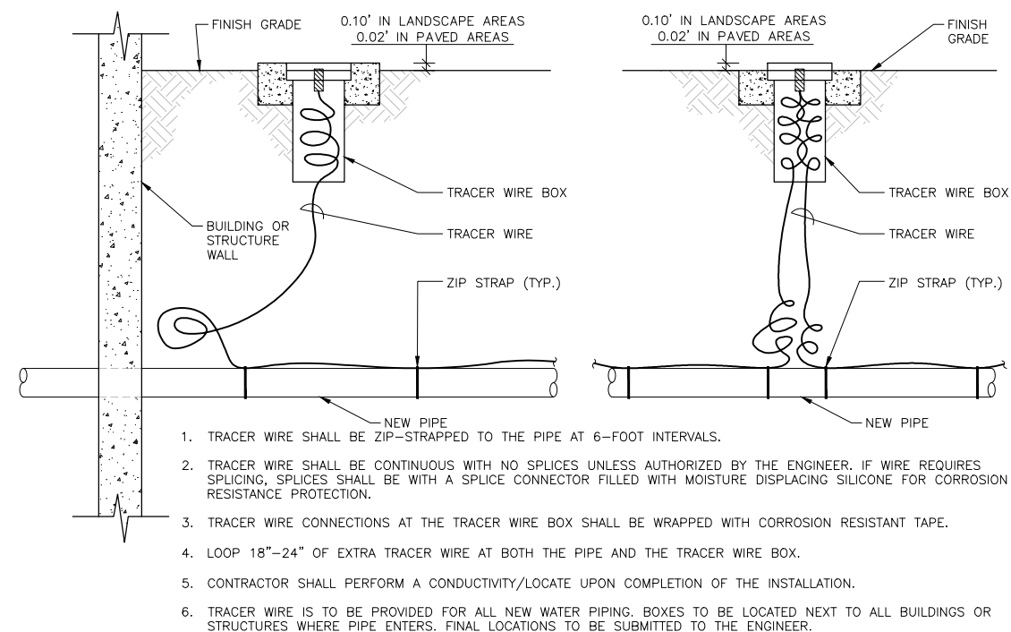
6 TRACER WIRE LOCATER BOX DETAIL NOT TO SCALE
