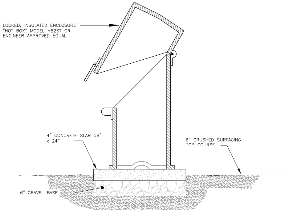
3 HOT BOX #2 - AIR GAP PIPING NOT TO SCALE
