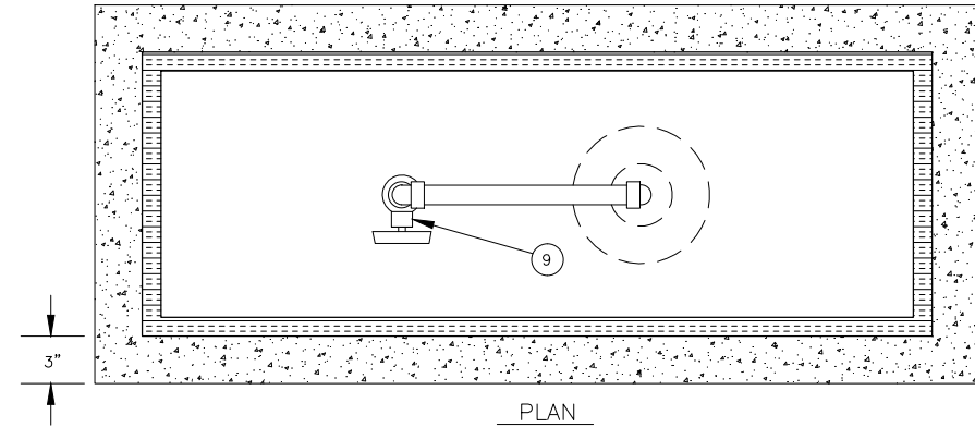
3 HOT BOX #2 - AIR GAP PIPING NOT TO SCALE
