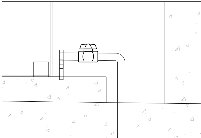
6 1" PVC BALL VALVE NOT TO SCALE
