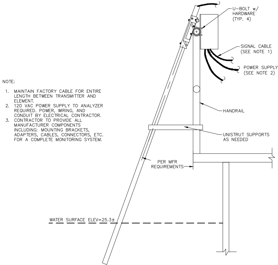
1 D.O. PROBE ELEVATION (TYP.) NOT TO SCALE
