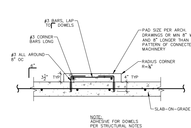
3 TYPICAL MECHANICAL EQUIPMENT PAD NOT TO SCALE
