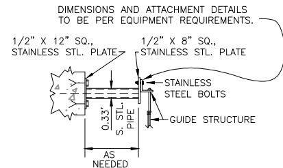
6 GUIDE STRUCTURE SUPPORT NOT TO SCALE
