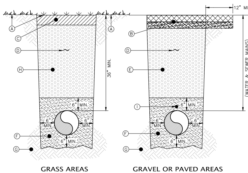
2 TYPICAL TRENCHING & BACKFILL NOT TO SCALE
