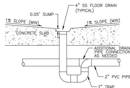
2 TYPICAL FLOOR DRAIN NOT TO SCALE
