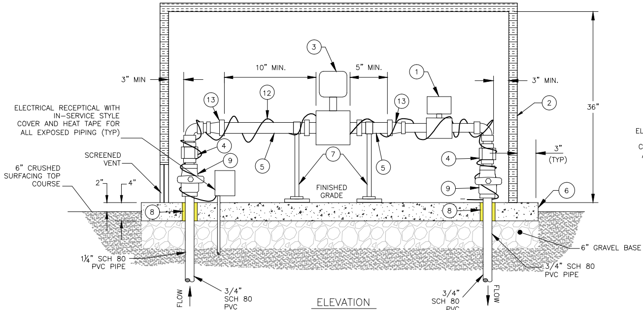
1 HOT BOX #1 - FLOW METER & ISOLATION VALVE NOT TO SCALE
