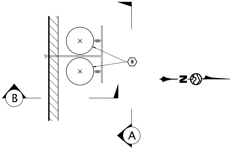
1 2W DIAPHRAGM TANKS – PLAN PIPE SUPPORTS NOT SHOWN FOR CLARITY 2 0 2 4 SCALE HORIZONTAL SCALE FEET
