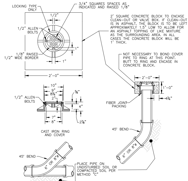
5 GRAVITY SEWER CLEANOUT DETAIL NOT TO SCALE
