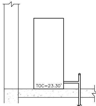
B 2W DIAPHRAGM TANK – SECTION 'B' VALVE HANDLES AND HOIST CHAINS NOT SHOWN FOR CLARITY.
