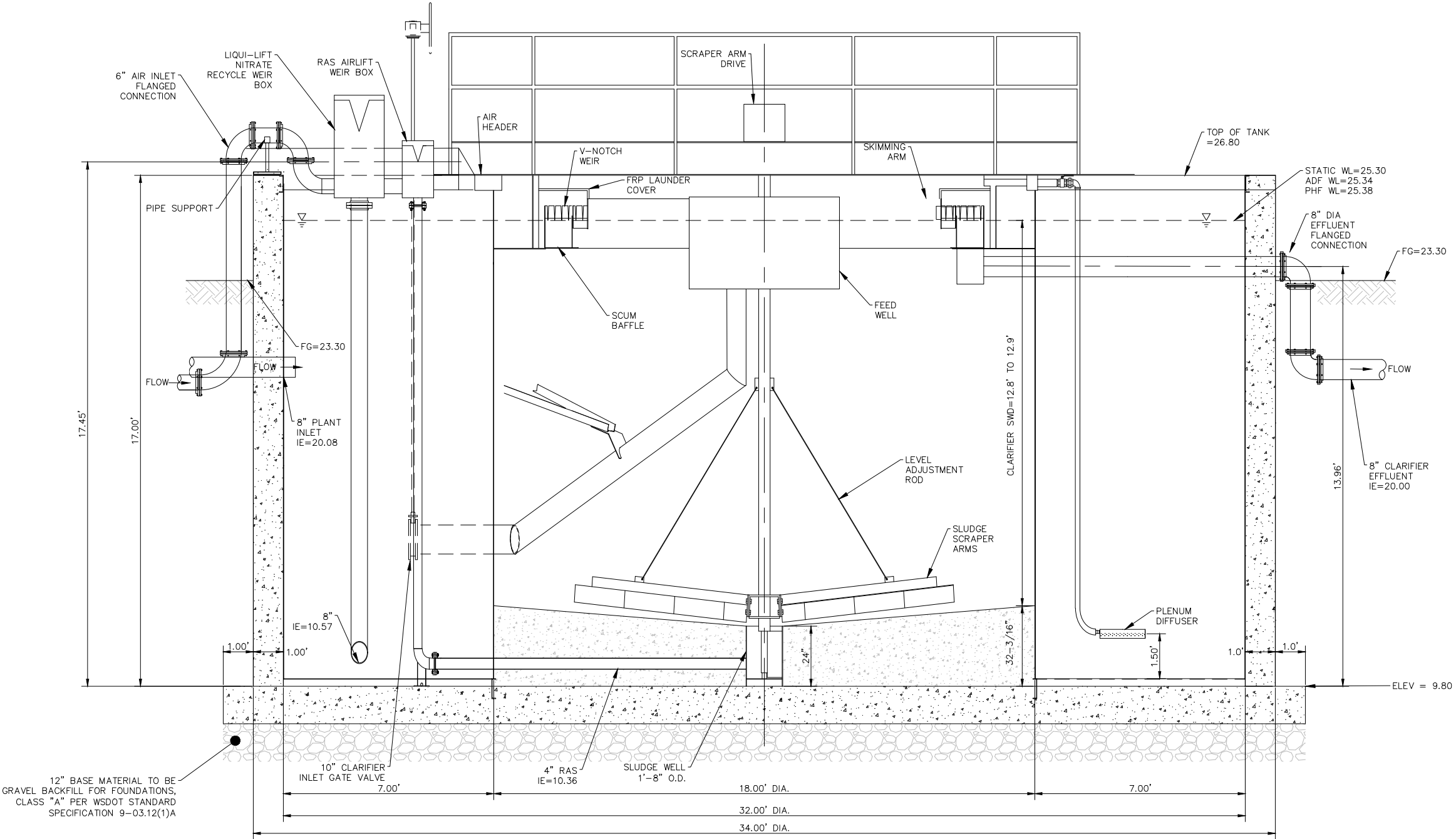
1 WEST-FACING SECTIONAL ELEVATION
