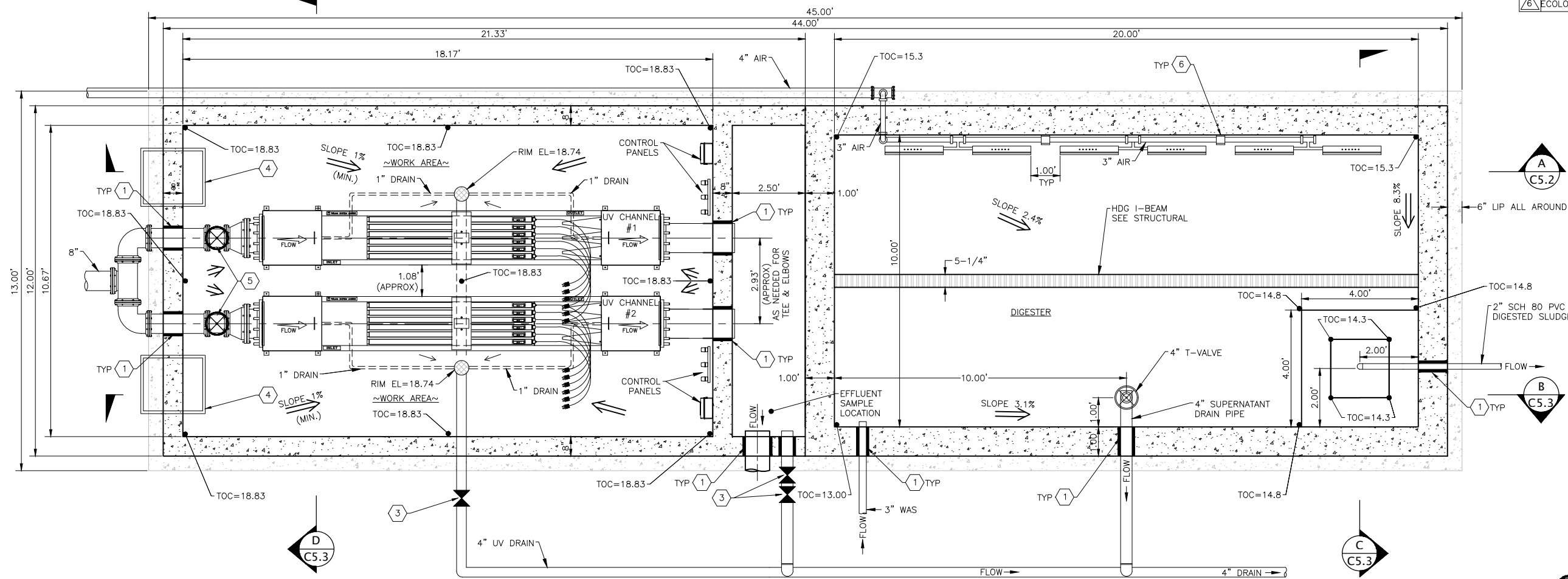
UV DISINFECTION CHAMBER & DIGESTER – PLAN VIEW
