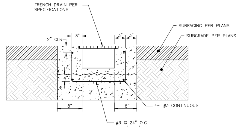
5 TRENCH DRAIN DETAIL NOT TO SCALE
