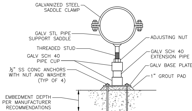
5 PIPE SUPPORT DETAIL NOT TO SCALE
