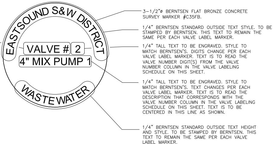
4 TYPICAL BURIED VALVE LABEL MARKER NOT TO SCALE
