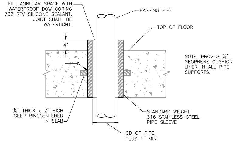
3 FLOOR SLEEVE DETAIL NOT TO SCALE
