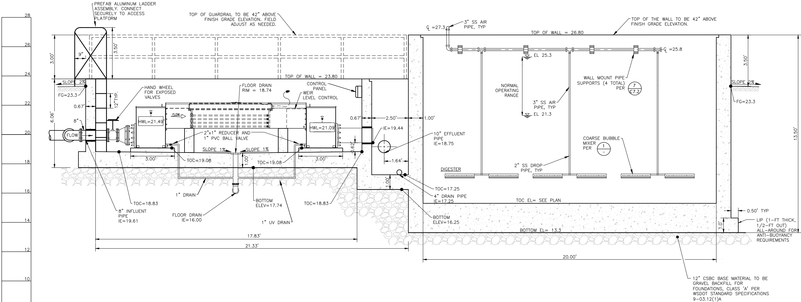
A UV DISINFECTION CHAMBER & DIGESTER - SECTION VIEW 'A' SCALE HORIZONTAL SCALE FEET
