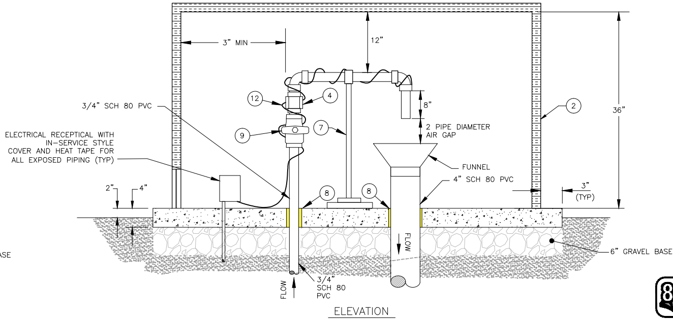
2 HOT BOX #2 - AIR GAP PIPING NOT TO SCALE
