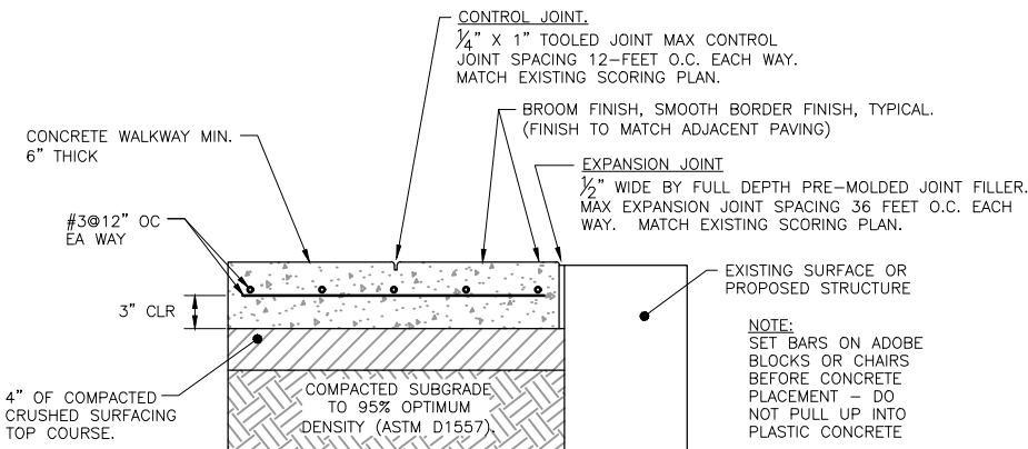
4 CONCRETE PAVEMENT DETAIL NOT TO SCALE
