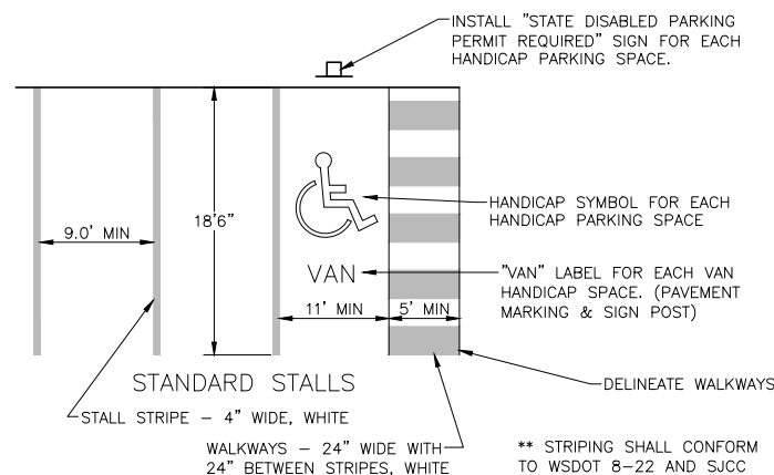
4 PARKING STALL STRIPING
