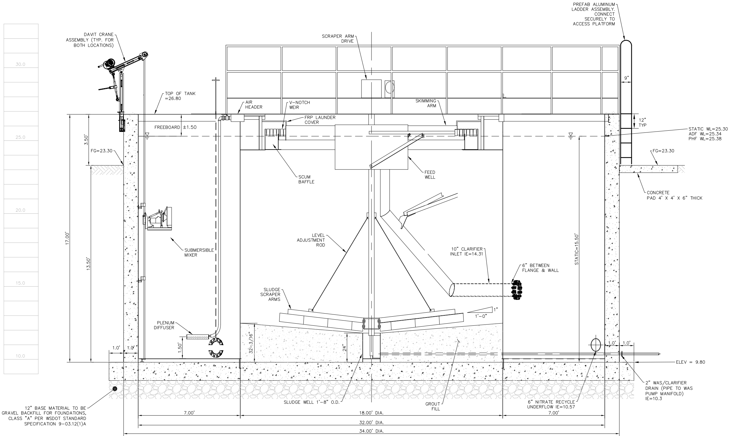
1 SOUTH-FACING SECTIONAL ELEVATION SCALE 0 2 4 FEET HORIZONTAL SCALE
